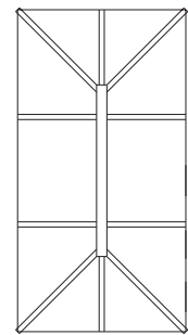
Maximum size Regular lantern as per this rafter layout 3000mm x 4000mm – can go up to 5000mm x 10000mm with additional rafters.
